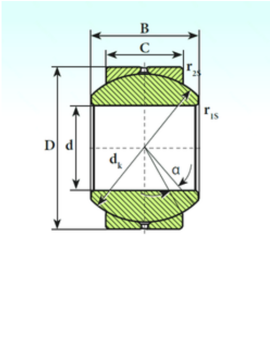
GE 6 SB Bearing 2D drawings and 3D CAD models
