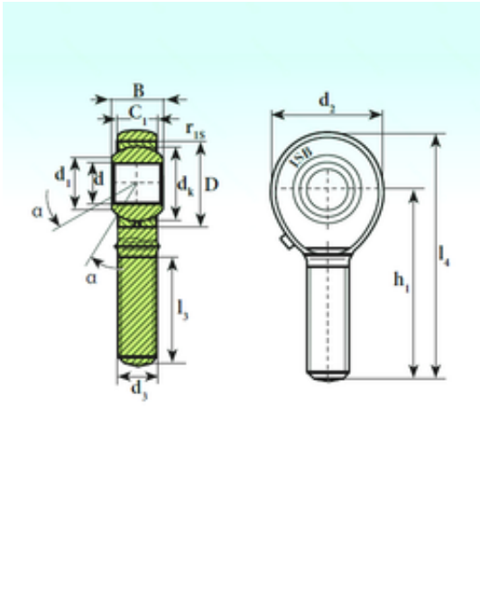
TSM 6 Bearing 2D drawings and 3D CAD models
